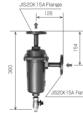
Drainage Trap DPM-15A Supplied by ITO. Painted grey
