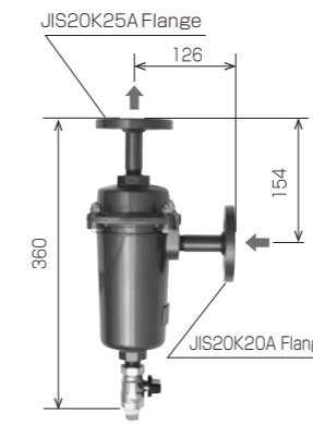
Drainage Trap DPM-20A Supplied by ITO. Painted grey
