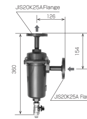
Drainage Trap DPM-25A Supplied by ITO. Painted grey
